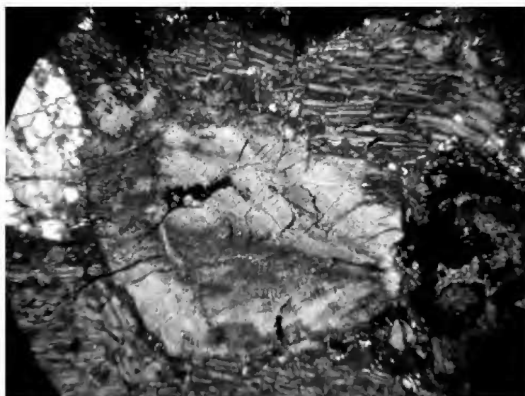
Fig.16- Transmitted crossed polarized light photomicrographs showing undulatory extinction on a pyroxene crystal. Length of field 0.4mm.
